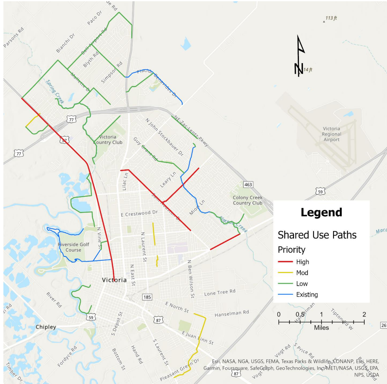
FIGURE A-2: SHARED USE FACILITY RECOMMENDATIONS BY PRIORITY
