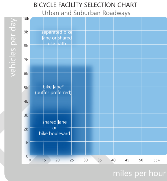
FIGURE 8. BICYCLE FACILITY SELECTION CHART
