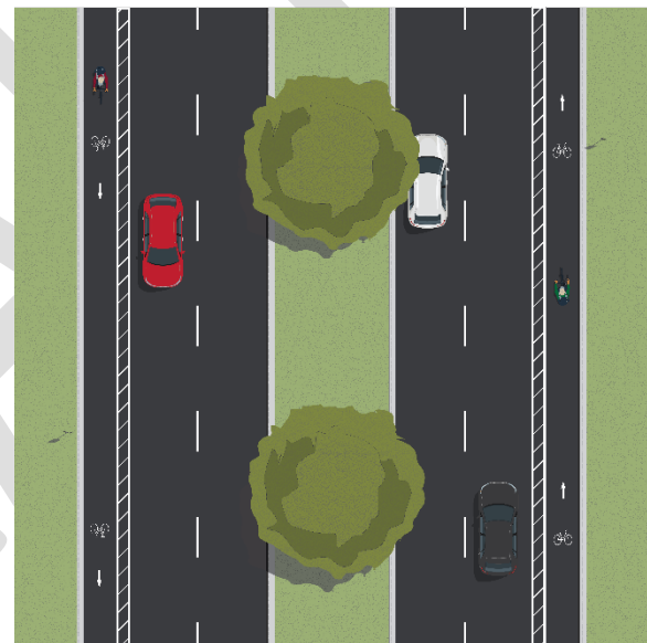
FIGURE 15. BUFFERED BICYCLE LANE
