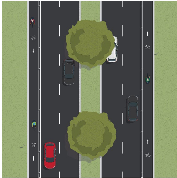
FIGURE 14. PROTECTED BICYCLE LANE
