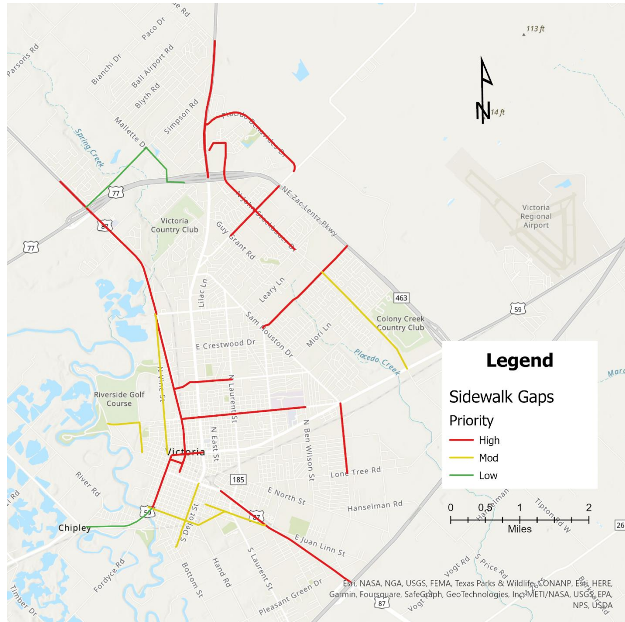
FIGURE A-3: SIDEWALK PROJECT RECOMMENDATIONS BY PRIORITY
