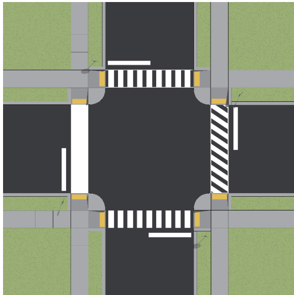
FIGURE 20. HIGH VISIBILITY CROSSWALKS
