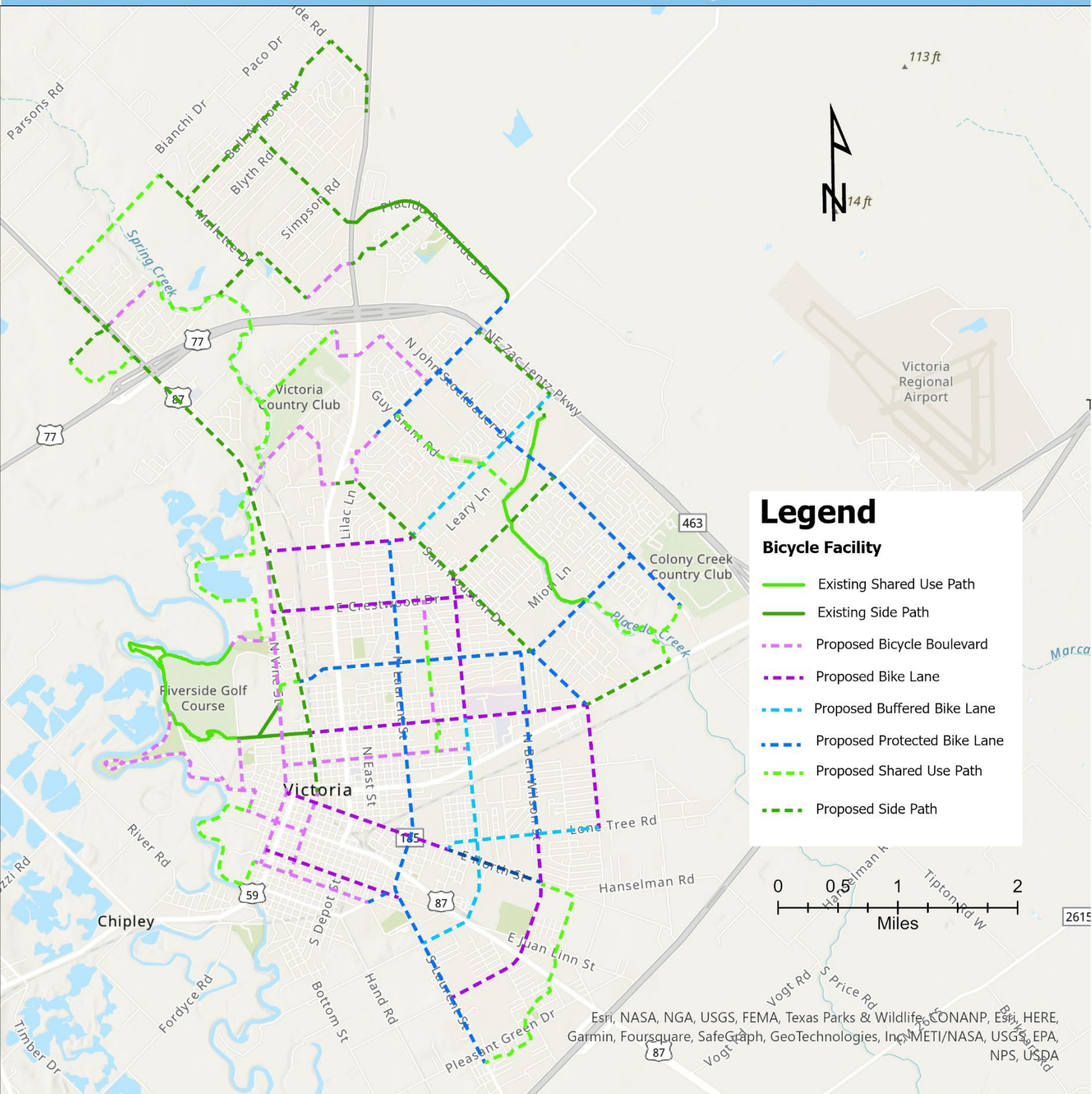
FIGURE 9. BICYCLE NETWORK RECOMMENDATIONS
