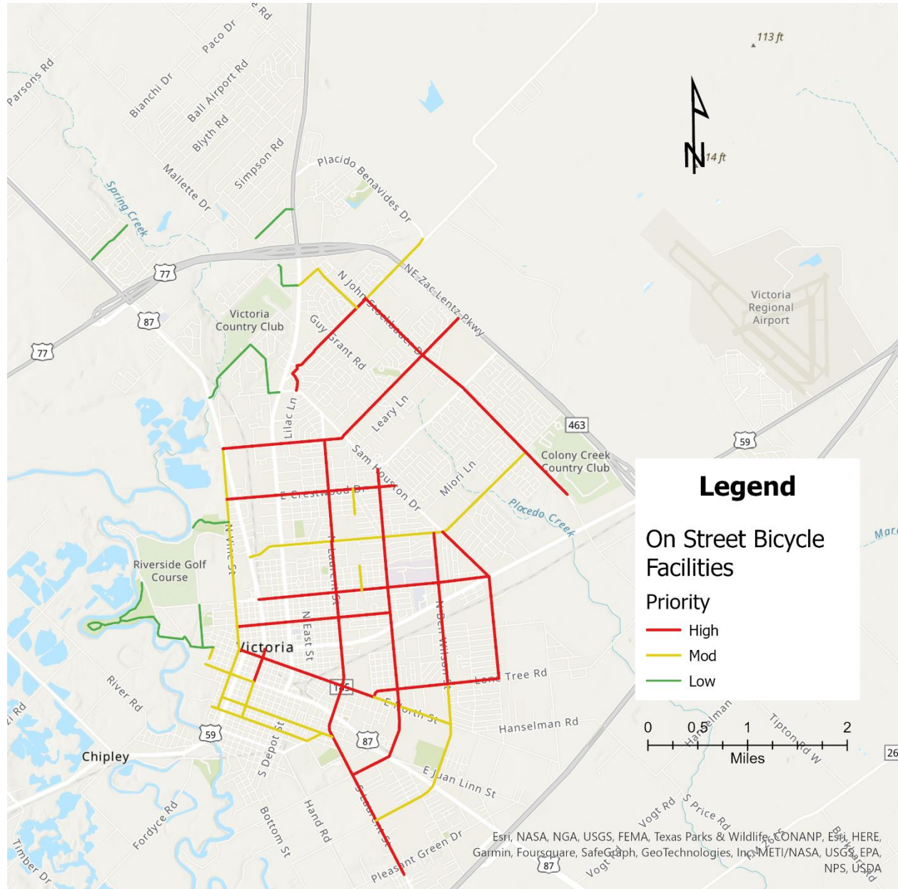
FIGURE A-1: ON STREET BICYCLE FACILITIES BY PRIORITY
