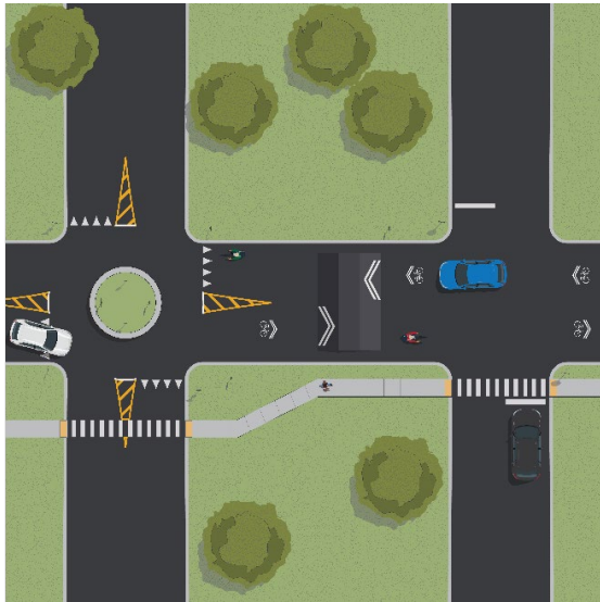
FIGURE 17. BICYCLE BOULEVARD
